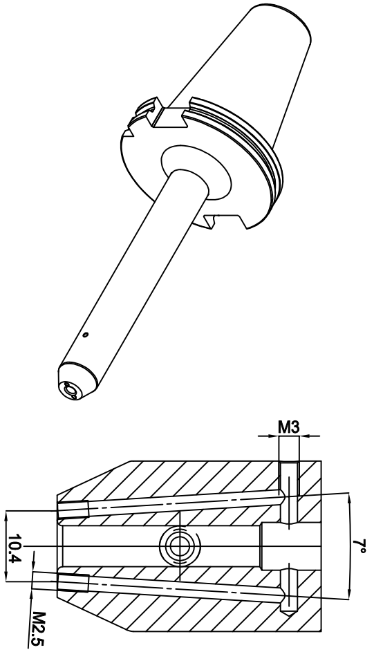
AA (2:1)
