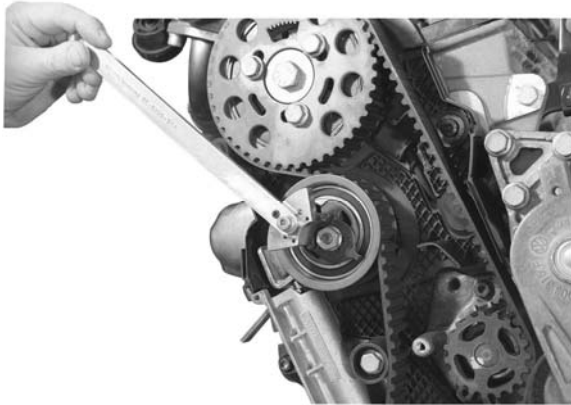
Tensioning the timing belt with the aid of KL-0284-91 A
