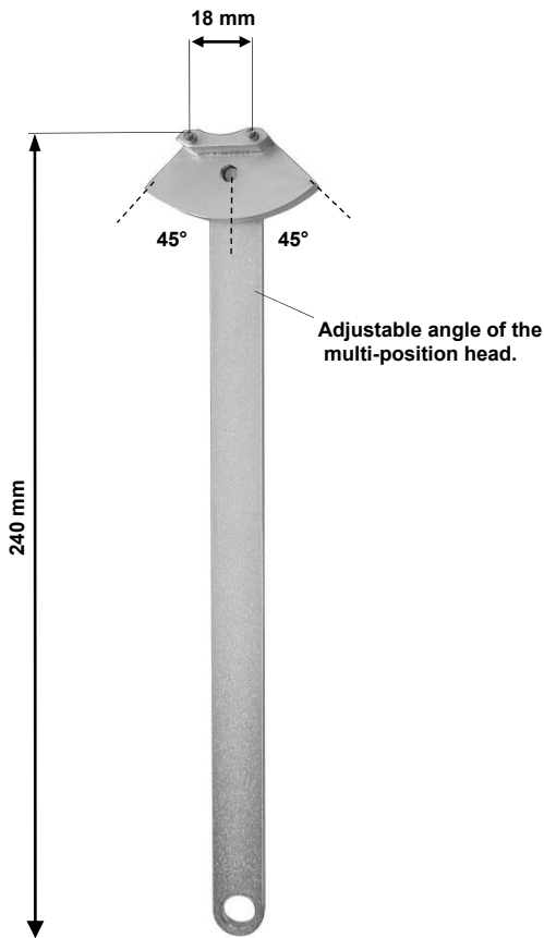
Tensioning the timing belt with the aid of KL-0284-91 A
