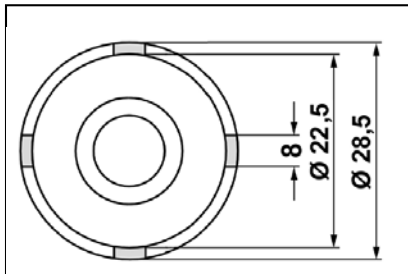
Dimensions KL-0369-601
