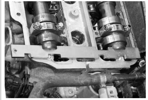
Locking the camshafts.
