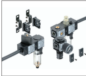
Comfort bloc. Quick component or combination change by means of connecting module (adhesive packing rings) shortens installation time.
